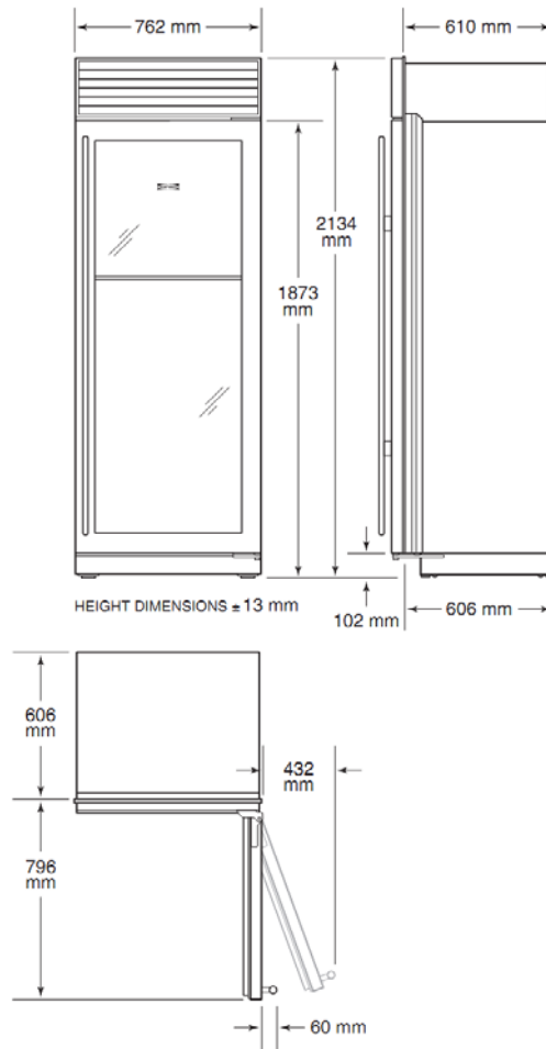
MODEL ICBWS-30
